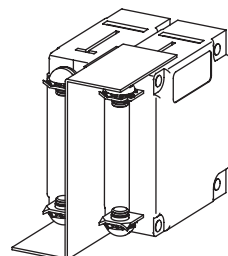
Optional "Z" Barrier
