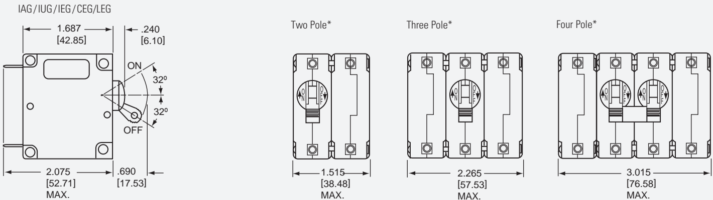
IAG/IUG/IEG/CEG/LEG Multi-Pole Circuit Breakers
