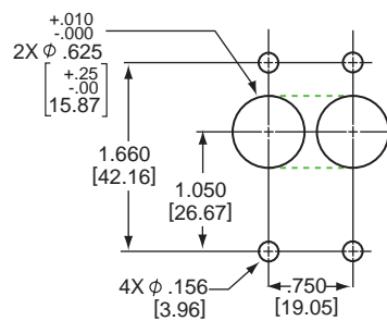
Two Pole
