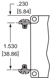
LEG Type Units Require Screw Terminals
