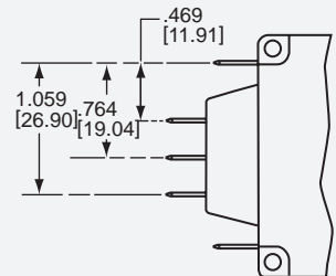
VDE Auxiliary Switch
