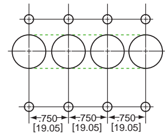
Four Pole*
